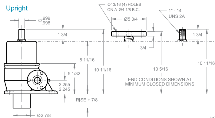
REDUCER DIMENSIONS
