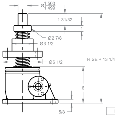
REDUCER DIMENSIONS
