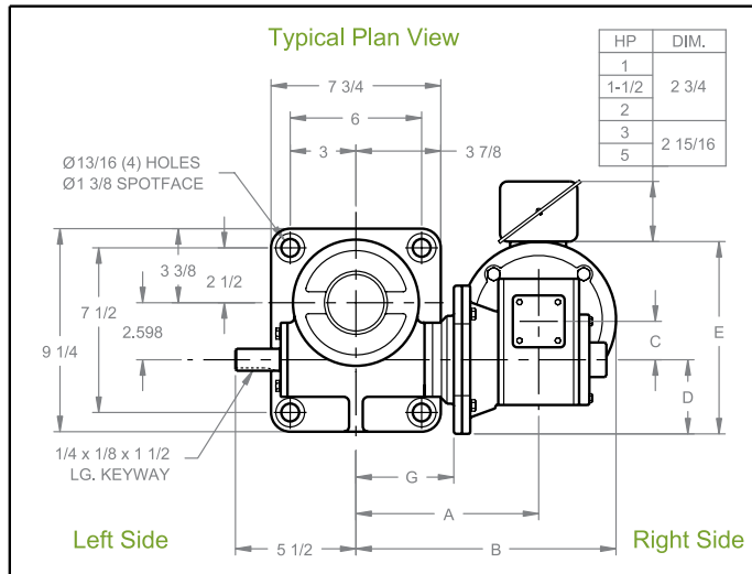
REDUCER DIMENSIONS
